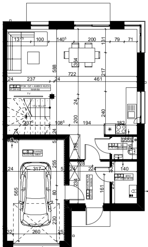
parter
