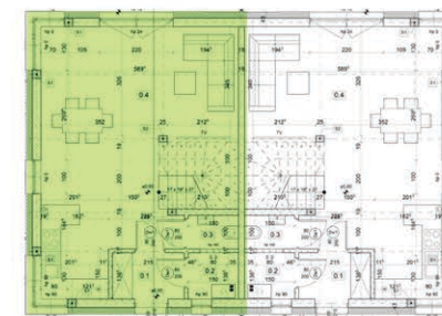
Parter
